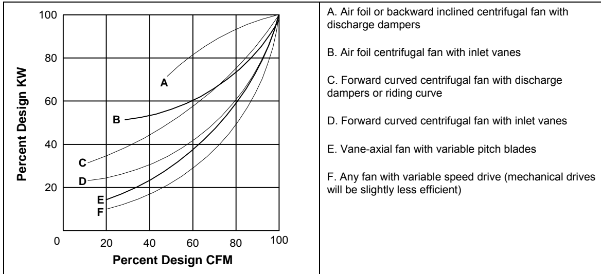
Figure 4-19 – VAV Fan Performance Curve
