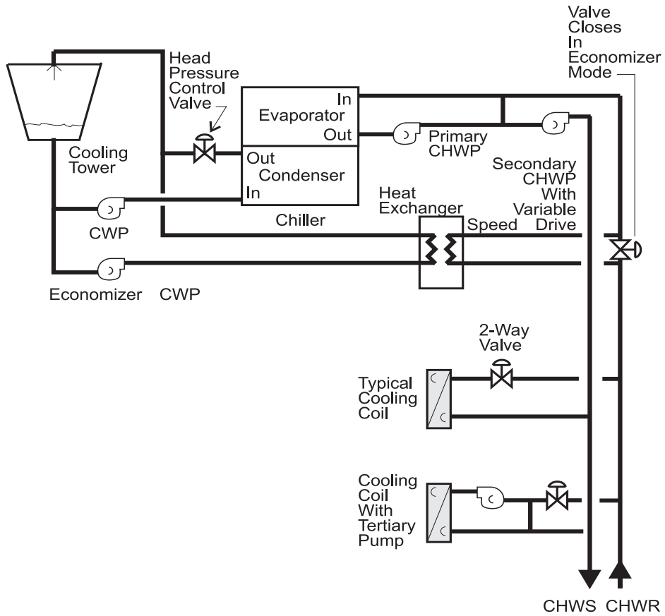
Figure 4-28 – Water-Precooling Water Economizer with Two-Way Valves
