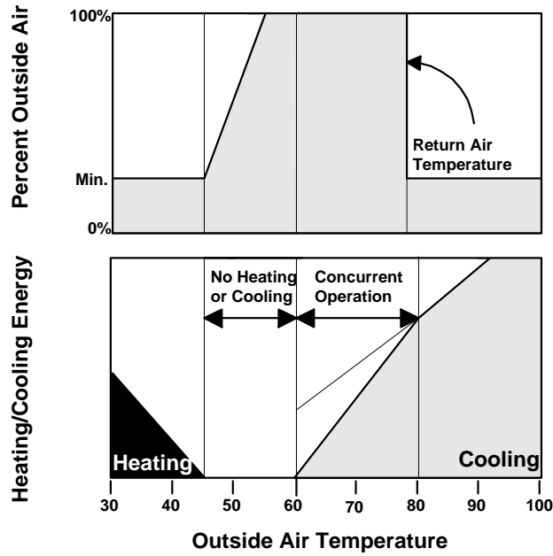
Figure 4-24 – Integrated Air Economizer
