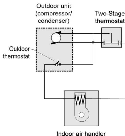
Figure 4-10 – Heat Pump Auxiliary Heat Control, Two-Stage and Outdoor Air Thermostats
