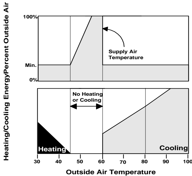
Figure 4-25 – Nonintegrated Air Economizer
