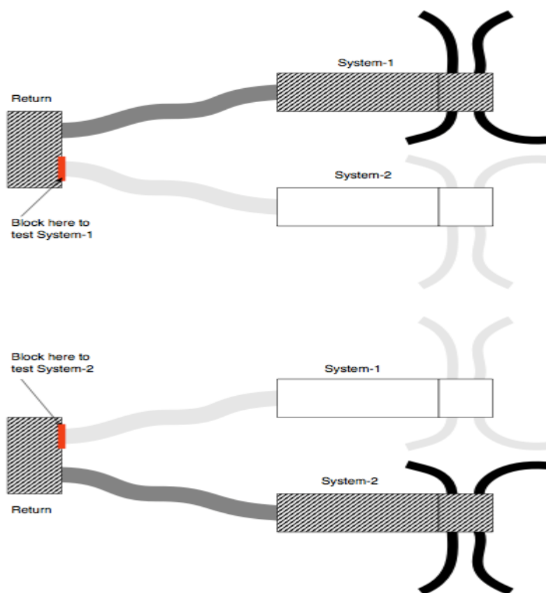
Figure 9 – Example of Two Duct Systems with a Common Return
