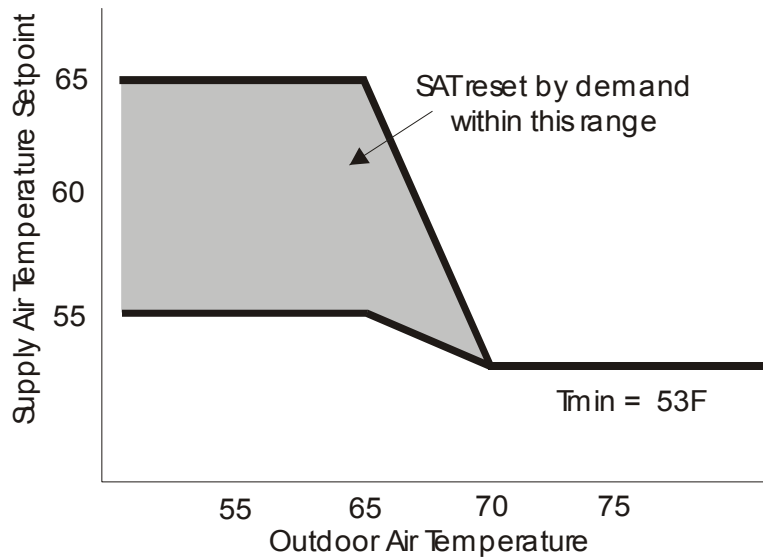
Figure 4-20 – Energy Efficient Supply Air Temperature Reset Control for VAV Systems Recommended Supply Air Temperature Reset Method
