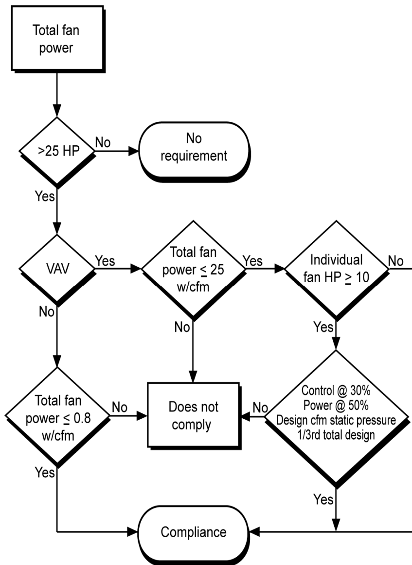
Figure 4-21 – Fan Power Flowchart
