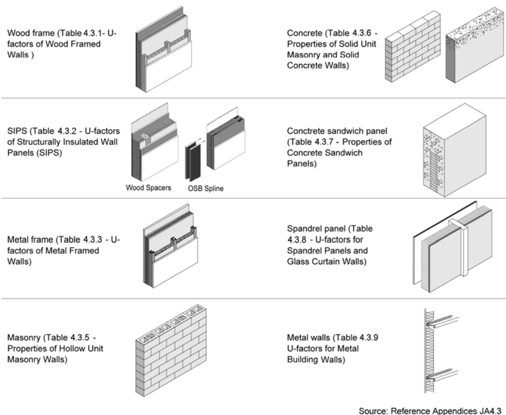
Figure 3-23 – Classes of Wall Constructions
