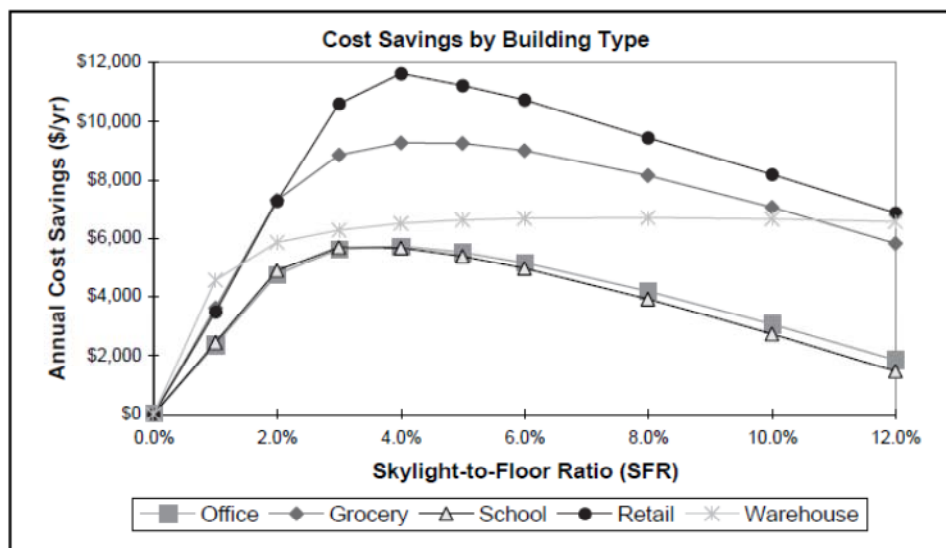
Figure 3-11 – Skylighting Savings by Skylight-to-Floor Ratio and Building Type in San Bernardino, CA (Climate Zone 10) 1
