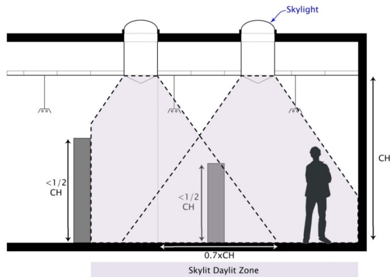
Figure 3-13– Daylit Area Tradeoff between Skylights and Windows
